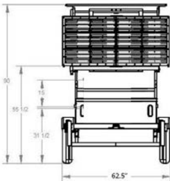
ATS Trailer: Stowed with SpeedAlert 24
