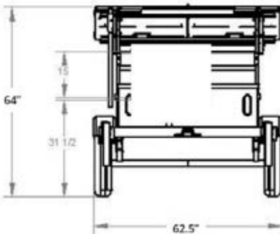
ATS Trailer: Stowed with SpeedAlert 24
