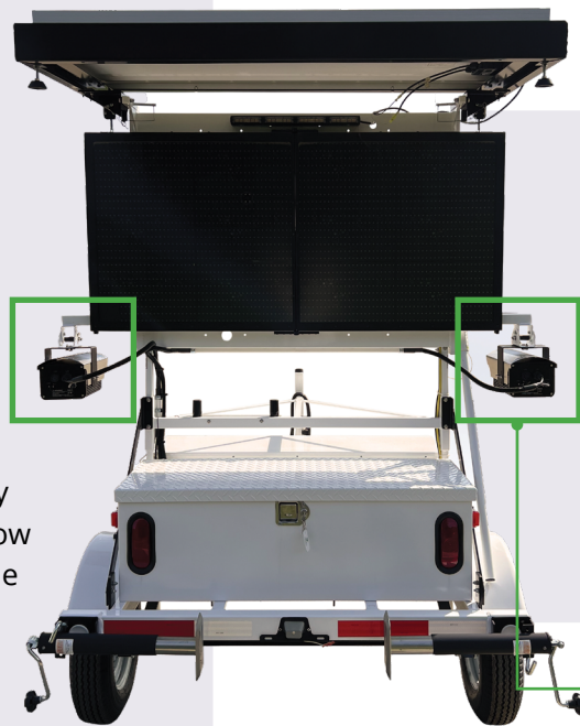
ELSAG M7 CAMERA SYSTEM IN CAMERA ENCLOSURE BOX
