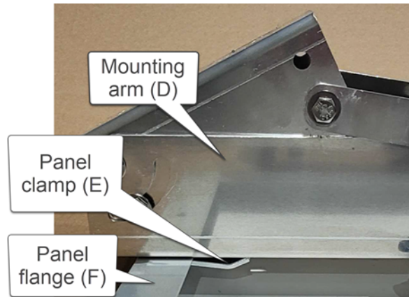
[Figure 10] Mounting arm, clamp, and flange
